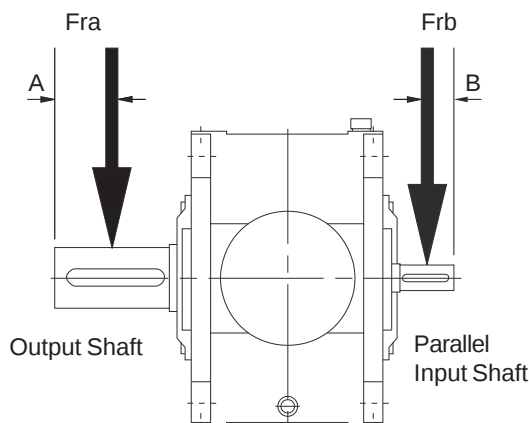
Output Shaft - Distance 'A' (midway along the shaft extension)
