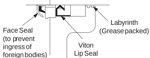
Standard Unit Output Shaft
