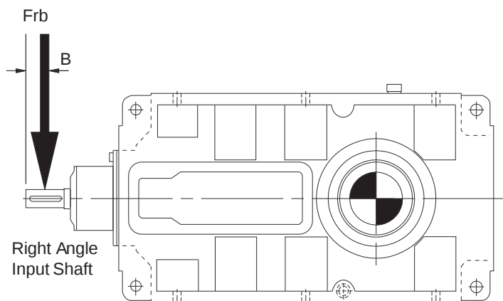
Input Shaft - Distance 'B' (midway along the shaft extension)
