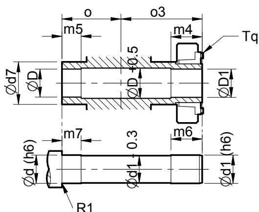
Shrink Disk
