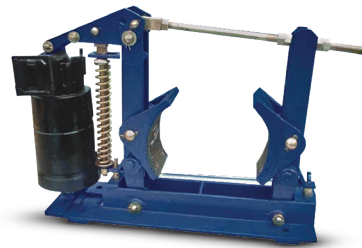
Electro Hydraulic Thrustor Brake
